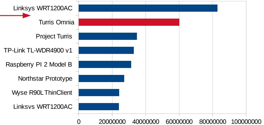
AES-128 benchmark
